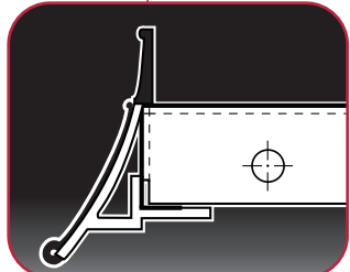
The shelves equipped with waterproof price-tag covers
