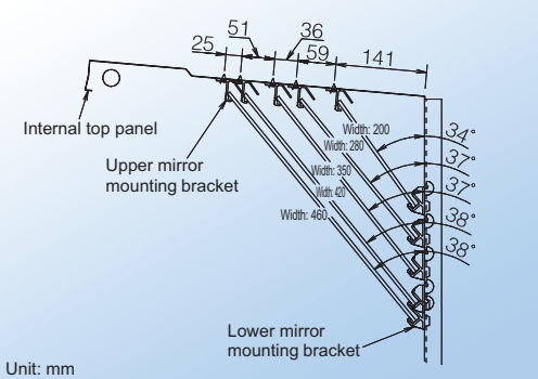
Mirror width and angle options FPW/CPW/CVS/FPS/CPS/CSM series
