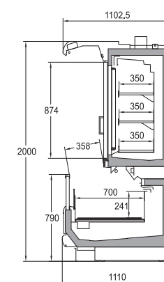
Select table for side-panel model Dual type freezer showcase (CZR series)
